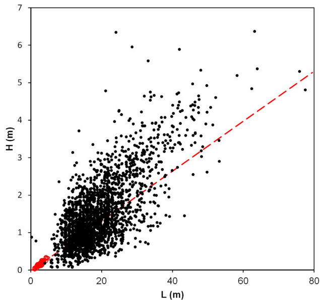
Fig. 12. MER-Opportunity ripple-like bedform length-height data from this study (red circles) plotted over summary data (black dots) redrawn from Fig. 5b of Hugenholz et al. (2017). Hugenholz et al. (2017) measured the heights and lengths (described by them as width) of many TARs using HiRISE DEMs. Red dashed line is the extrapolated linear regression derived from our measurements shown in Fig. 8b. (For interpretation of the references to colour in this figure legend, the reader is referred to the Web version of this article.)
